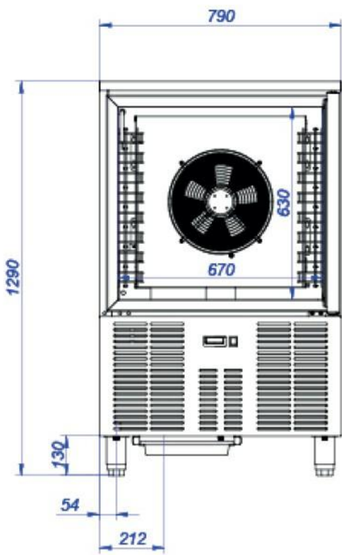
SP0840BC Dimensions
